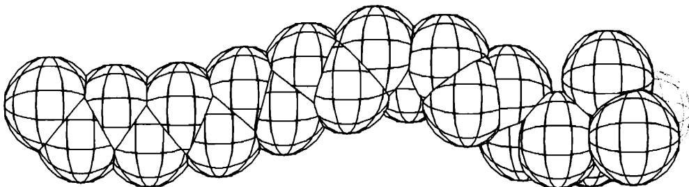
Figure 2. SPACEFILL representation of stearyl dimethylamine oxide.
