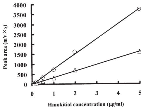
Figure 3. Standard curves of hinokitiol. (O) at 240 nm. (Δ) at 345 nm.
