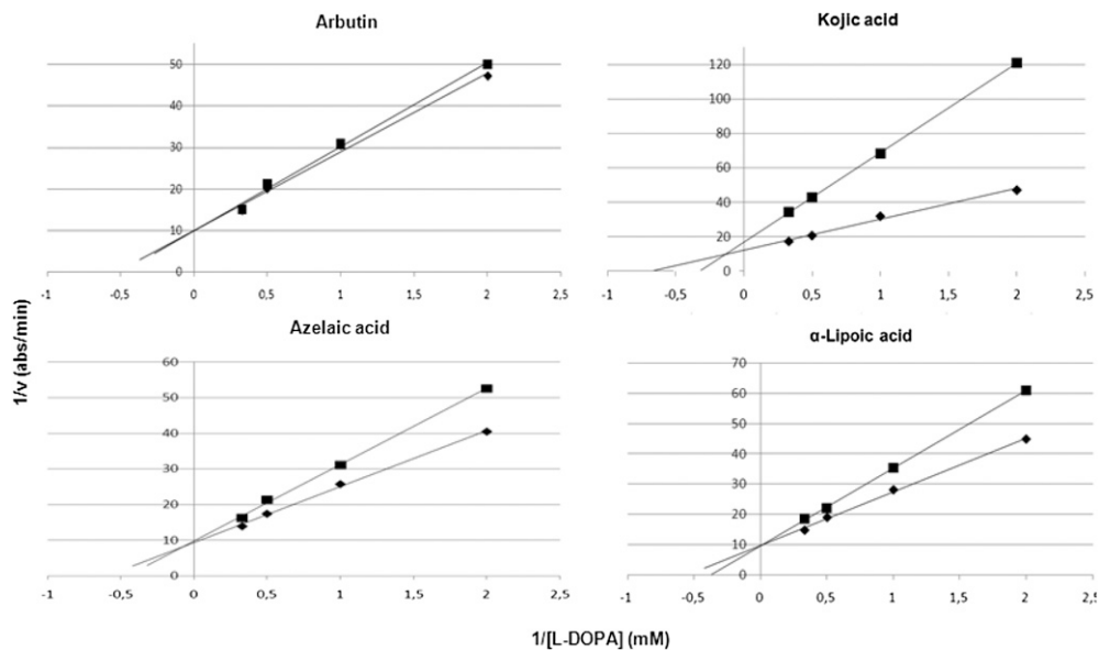
Figure 4. Lineweaver–Burk plots of mushroom tyrosinase. Arbutin (500 µg/ml), kojic acid (10 µg/ml), azelaic acid (100 µg/ml), and α- lipoic acid (50 µg/ml) were incubated with 0.5, 1, 2, and 3 mM L-DOPA.
