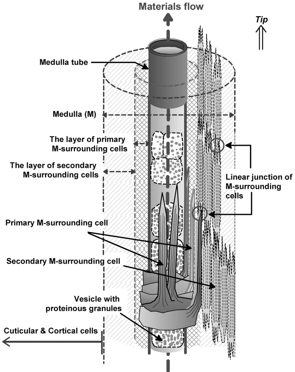
Figure 6. Schematic representation of the M of a human scalp hair fiber. One end of the primary M-surrounding cell is attached to the M tube, whereas the other end is bound to the secondary M-surrounding cell; cf. Figure 5A. The secondary M-surrounding cell also forms a linear junction with the other secondary M-surrounding cell. Hence, all of the M-surrounding cells are bound directly or indirectly to the tube wall, covering around the tube. In general, adults' M tube, unlike an elderly persons' tube, is neatly packed with the vesicles which are full of proteinous granules (0.5–1 \mu\text{m} in diameter). Various materials in aqueous solution may flow through the tube.
