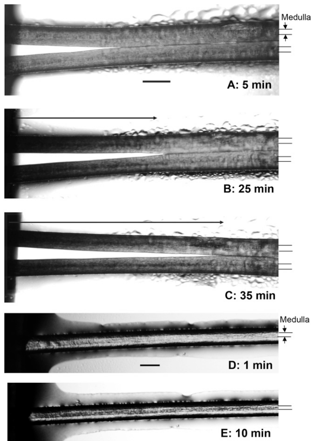
Figure 11. (A–C) The \text{H}^+ ion-flow through the M of the black hair fiber (jf8) at 25^\circ\text{C} ; bar 100 \mu\text{m} . The fiber was thoroughly stained with Congo red, then its left end was acidified by 0.5 M HCl; see the procedure “ \text{H}^+ ion-flow through the M: The use of Congo red as an indicator” for more details. The time-lapse after acidification is printed in each picture. The M changed gradually in color from gray to reddish black toward the right hand side, as indicated by the arrow. The M tube was isotropic to the flow of \text{H}^+ ions. (D and E) The \text{OH}^- ion-flow through the M at 25^\circ\text{C} ; bar 100 \mu\text{m} . The white hair fibers (jm67) were stained by an aqueous solution of phenolphthalein, and then one of the two ends was alkalinized by 1 M NaOH; cf. the procedure “ \text{OH}^- -flow through the M: the use of phenolphthalein as an indicator” of the experimental section. The color change (to red) occurred only in the M, taking less than 10 min to extend to the other end.
