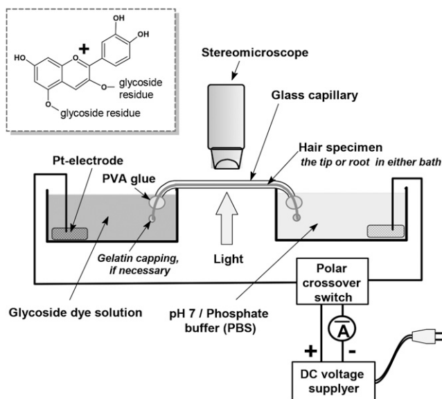
Figure 3. The instrumental setup for the DC voltage-assisted flow of the purple anthocyanin dye. The white hair fiber was put into a glass capillary, and the fiber ends were dipped into the electrode solutions as depicted in the figure. An aqueous solution of the cationic dye and the buffer solution were initially set as the positive and the minus electrode solutions, respectively; see the procedure “Flow of the anthocyanin dye through M: Application of a DC voltage to a hair shaft” for more details.
