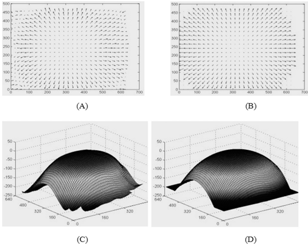
Figure 5. Needle maps and reconstructed results of the ball bearing from the Skin Analyzer and theoretic results calculated from an ideal sphere model.
