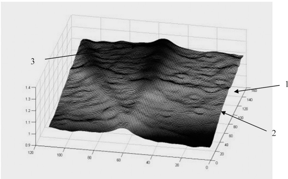
(B) 3D reconstructed result from surface gradient data taken from photometric stereo
