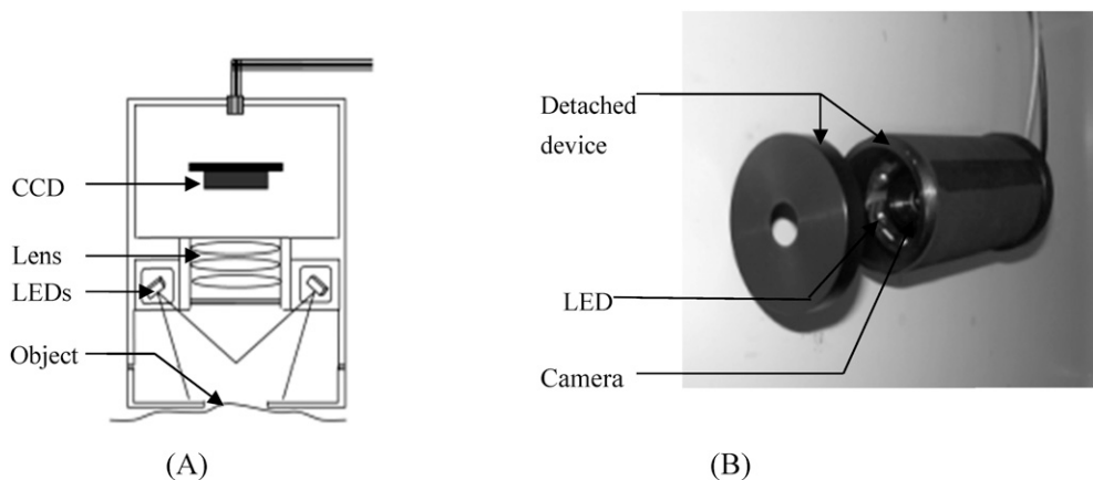
Figure 1. Schematic (A) and developed (B) handheld skin lesion imaging system – known as the “Skin Analyzer” composed of a small IEEE1394 digital camera (AVT Marlin, F-046C) and a high-resolution compact lens (Schneider, 1.4/23 mm + extension tube), surrounded by six surface-mounted high power chip-type LEDs (NSCW455, NICHIA, Tokushima, Japan) positioned equidistantly in angle on a circle of radius 8 cm that is centered on the camera’s optical axis and lies in a plane orthogonal to this axis in line with the front of the first optical element of the lens.
