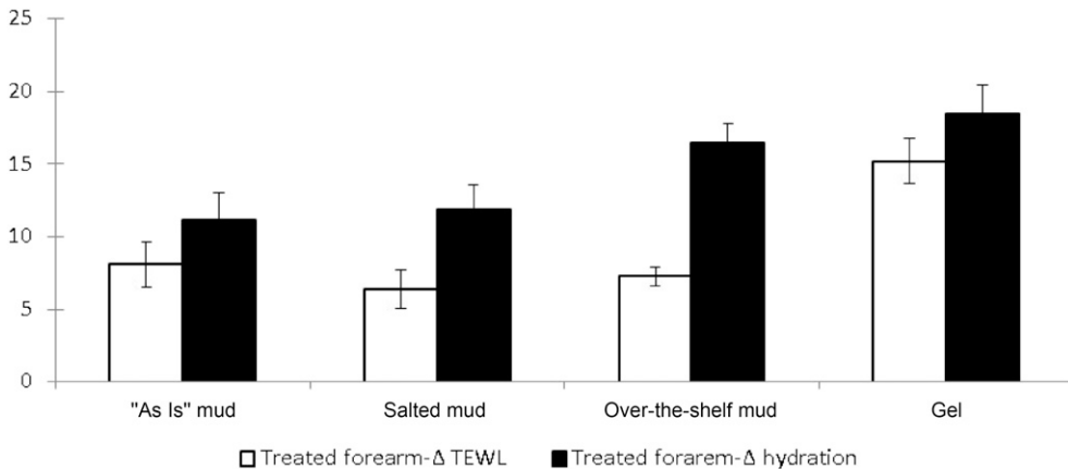
Figure 4. Changes in skin hydration ( \Delta hydration) and TEWL ( \Delta TEWL) from baseline values for forearms treated with "As Is" mud ( n = 20 ), salted mud ( n = 20 ), over-the-shelf mud ( n = 20 ), and gel ( n = 15 ) directly after mud removal. Values represented as mean \pm SEM.
