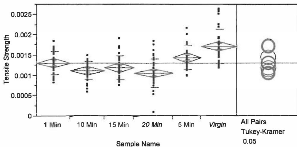
Figure 2. Statistical analysis for tensile strength measurement.
