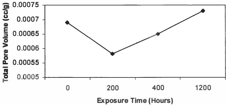
Figure 13. Pore volume (cc/g) versus UV irradiation times of 0, 200, 400, and 1200 hr.
