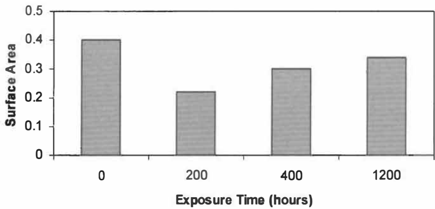
Figure 12. Surface area (m²/g) versus UV irradiation times of 0, 200, 400, and 1200 hr.
