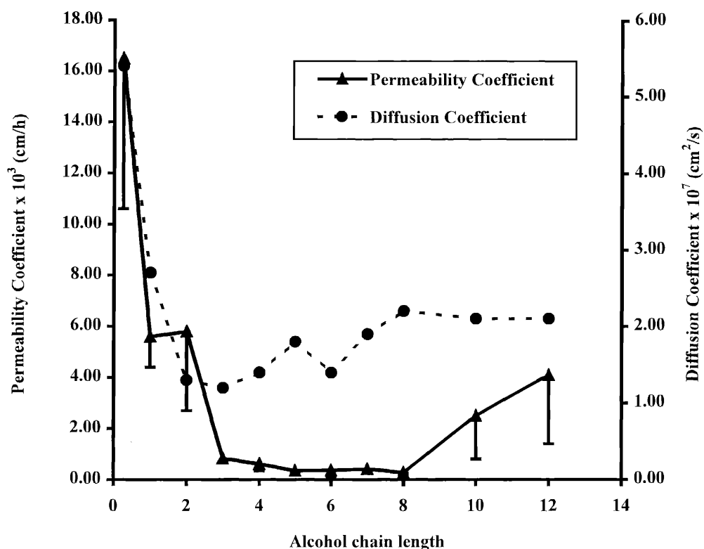
Figure 2. Effect of chain length on the permeability coefficients and diffusion coefficients of a series of diluted, homologous n -alkanols through the human nail plate. Mean \pm S.D., n = 4 –26. Adapted from reference 33.
