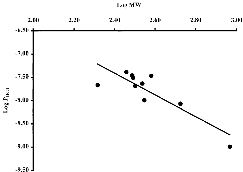
Figure 3. Relationship between the logarithm of molecular weight (MW) of various antimycotics and the logarithm of their permeability coefficients through a bovine hoof membrane ( P_{Hoof} ). Adapted from reference 37.
