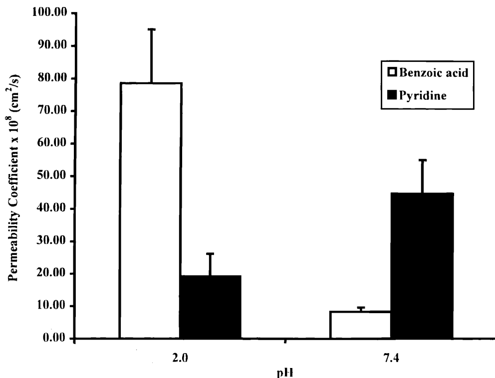
Figure 4. Effect of pH on the permeability coefficients of benzoic acid and pyridine through a bovine hoof membrane. Mean \pm S.D., n = 4 . Adapted from reference 36.
