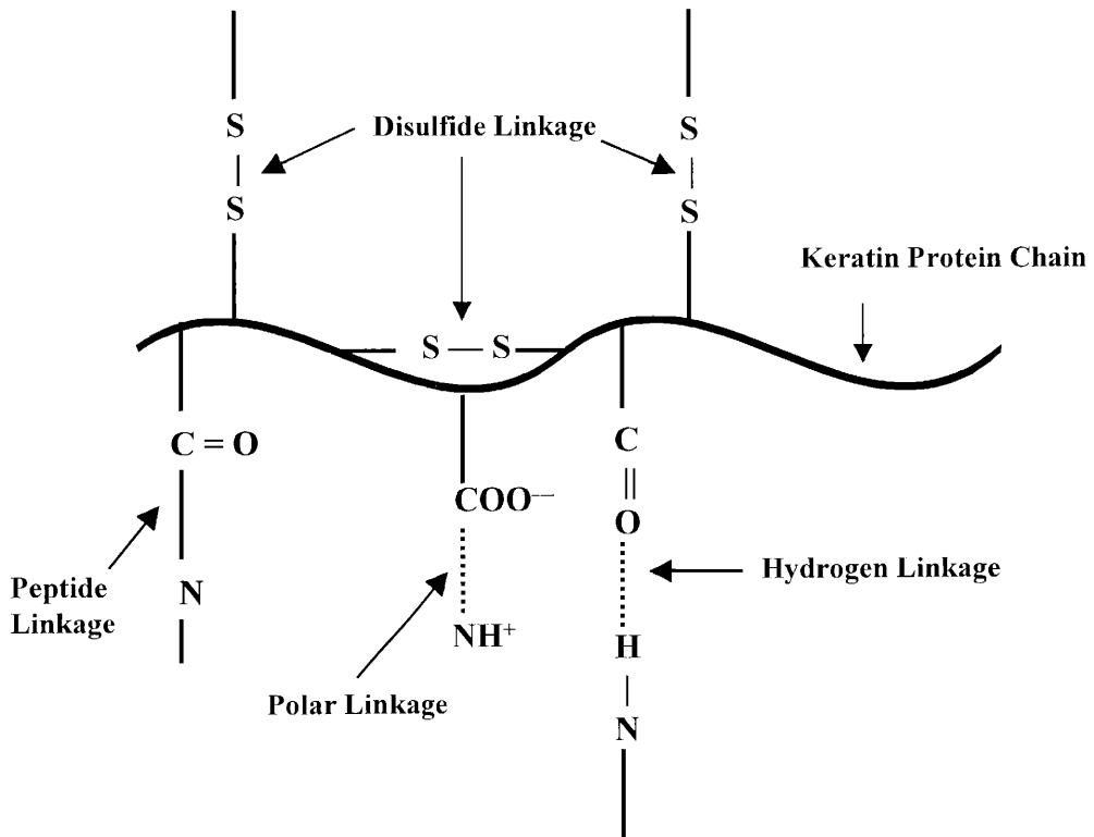
Figure 5. Schematic representation of the bonds in nail keratin that represent potential interaction sites for nail penetration enhancers. Adapted from reference 5.
