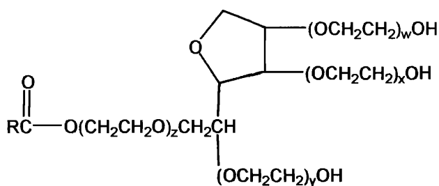
polysorbate 20, R=C_{11}H_{23} ; polysorbate 60, R=C_{17}H_{35} ; polycorbate 80, R=C_{17}H_{33}
