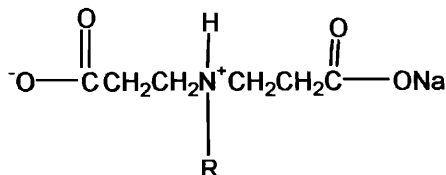
sodium alkyl iminodipropionate
