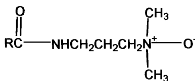
alkylamidopropylamine oxide
