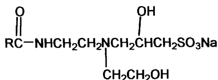
sodium alkylamphohydroxypropylsulfonate
