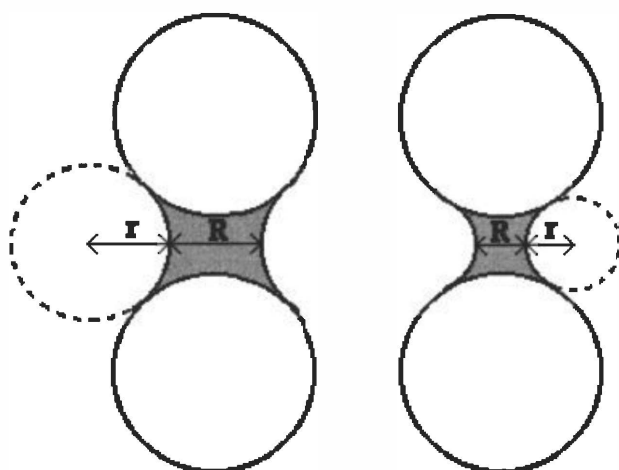
Figure 5. Schematics of the oil liquid bridge between two fibers. Oil penetration decreases the contact area, A = \pi R^2 , and increases the Laplace pressure, P = \sigma \cos \theta / r , where \sigma is the surface tension of oil and \theta is the contact angle. The combined effect of these two results in a decrease in adhesive force ( P_1 A_1 > P_2 A_2 ).
