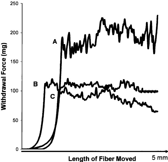
Figure 4. Typical withdrawal force curves for Indian hair fibers treated with sunflower oil after 5 minutes (A), after 24 hours (B), and after 24 hours with heat treatment (C). Curves shifted arbitrarily.
