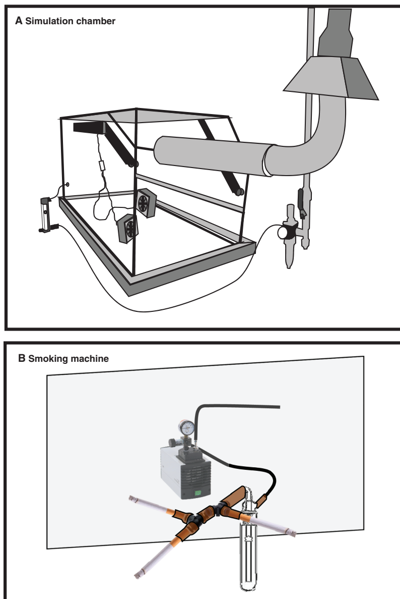
Figure 1. Scheme of (A) the developed exposition chamber and (B) smoking machine used to perform dermal absorption studies of hazardous organic compounds from cigarette smoke.
