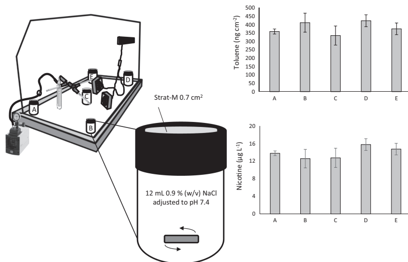
Figure 2. Scheme of the modified vertical Franz diffusion cell and used in this study and results obtained from the five evaluated points inside the simulation chamber to evaluate air homogeneity.
