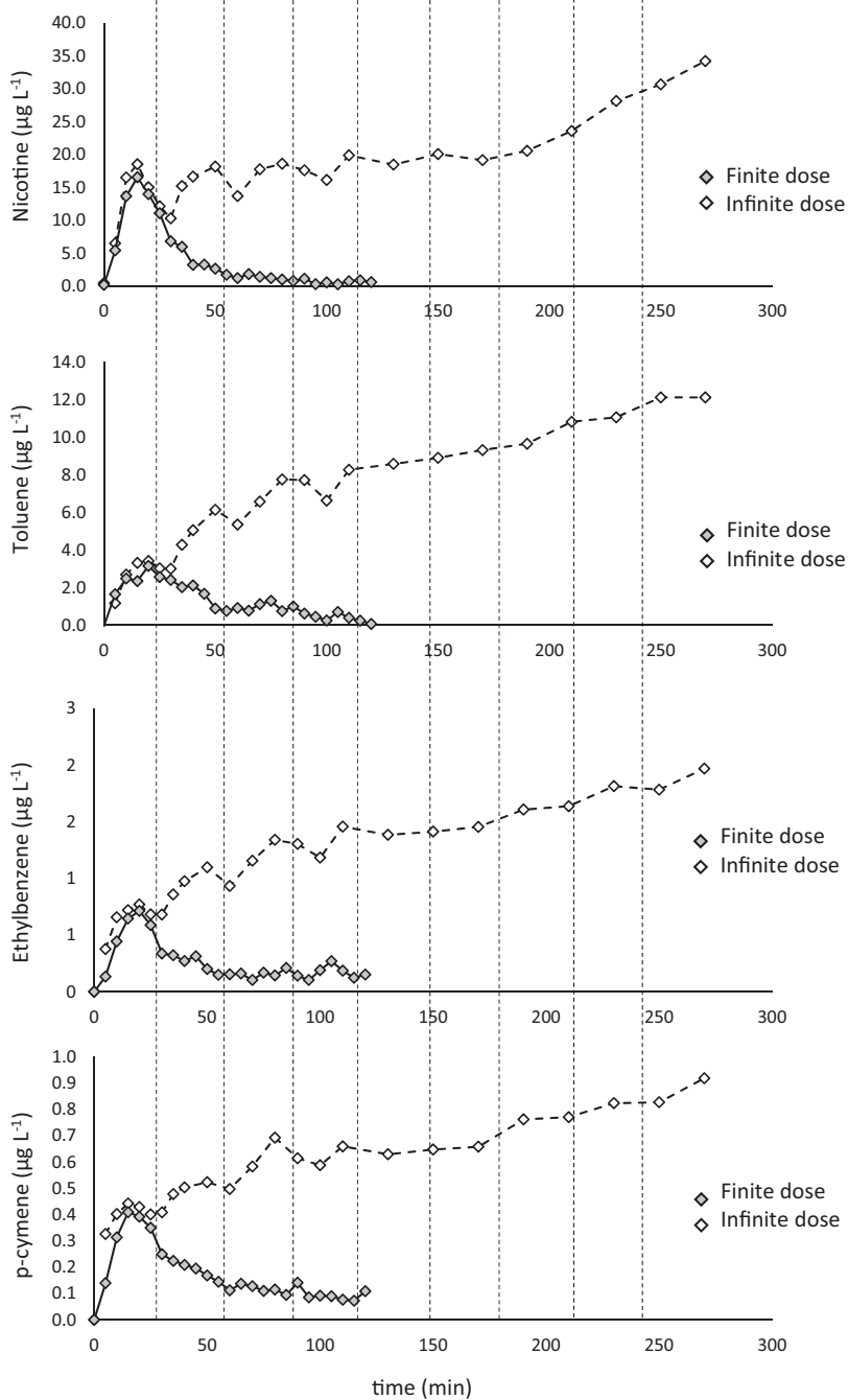
Figure 3. Concentration profile of selected hazardous organic compounds from cigarette smoke inside the simulation chamber measured by active sampling in finite (grey dots) and infinite (white dots) dose conditions.
