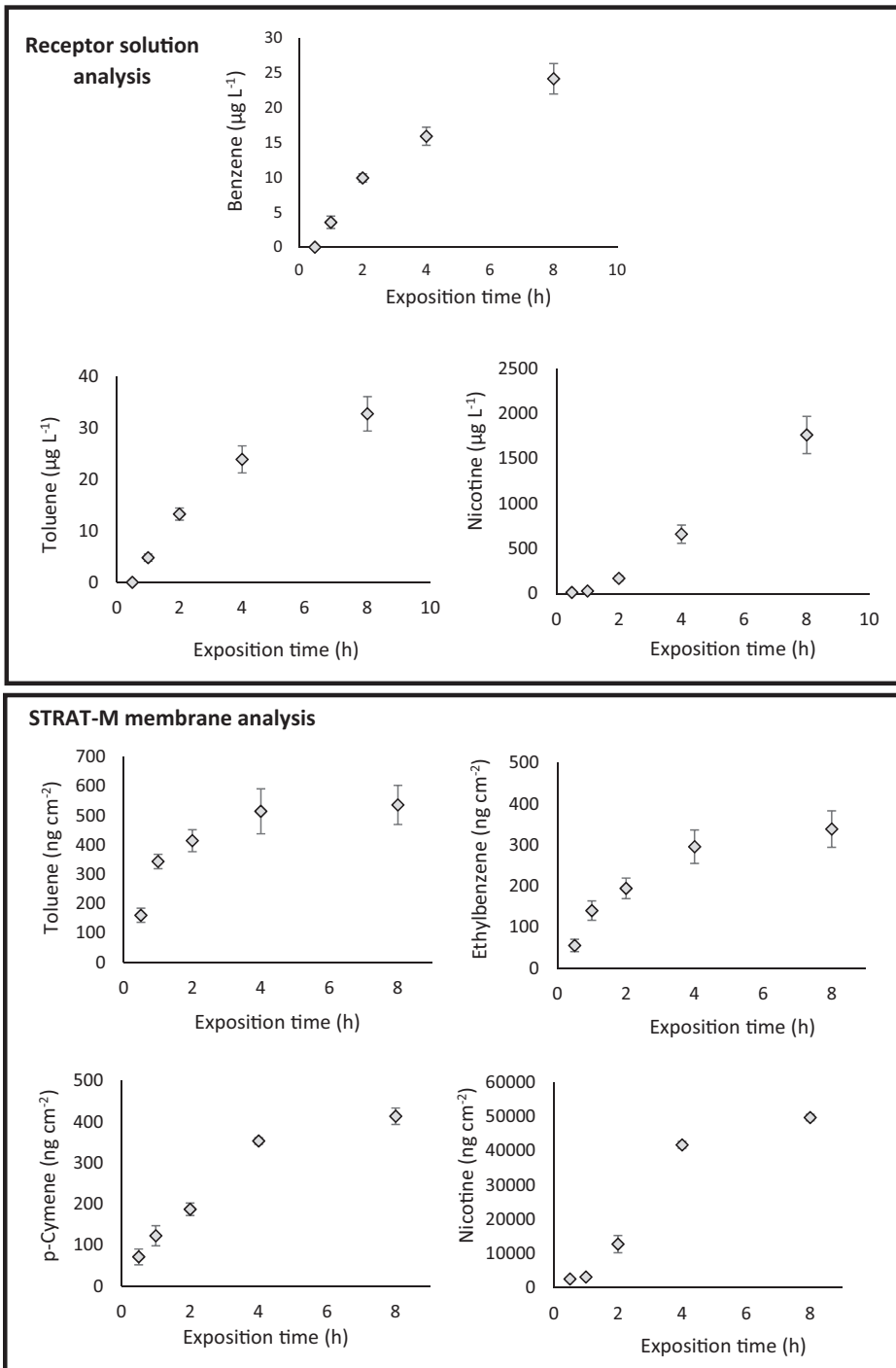
Figure 5. Dermal absorption studies of selected hazardous organic compounds from cigarette smoke in infinite dose conditions.
