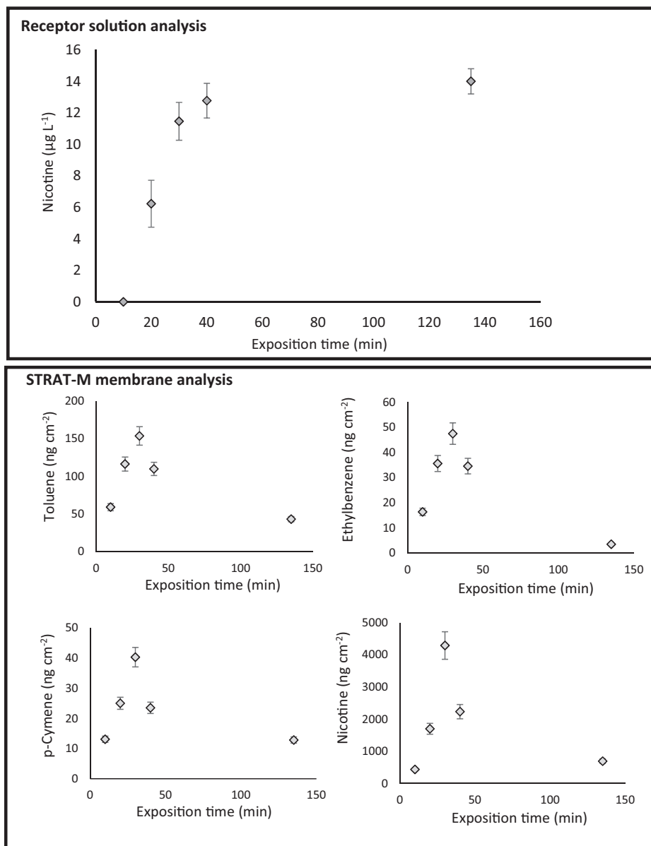
Figure 4. Dermal absorption studies of selected hazardous organic compounds from cigarette smoke in finite dose conditions.
