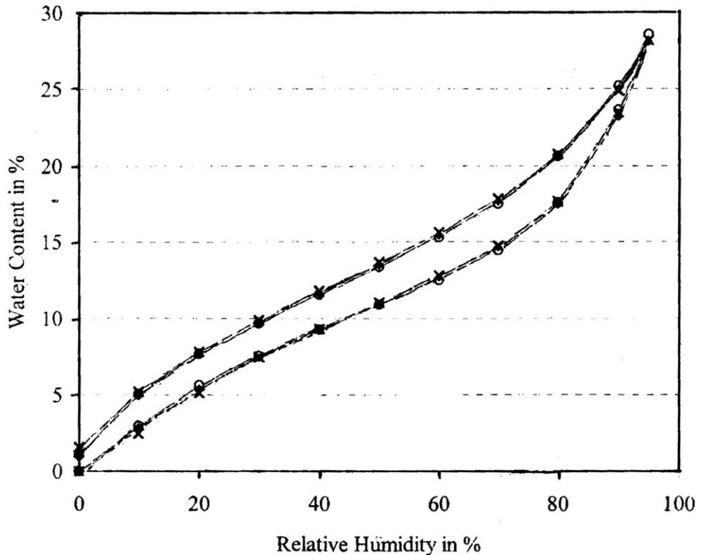
Figure 1. Hair–water S–D isotherms for untreated hair. Expt. 1: ◇; Expt. 2: ○; Expt. 3: x.
