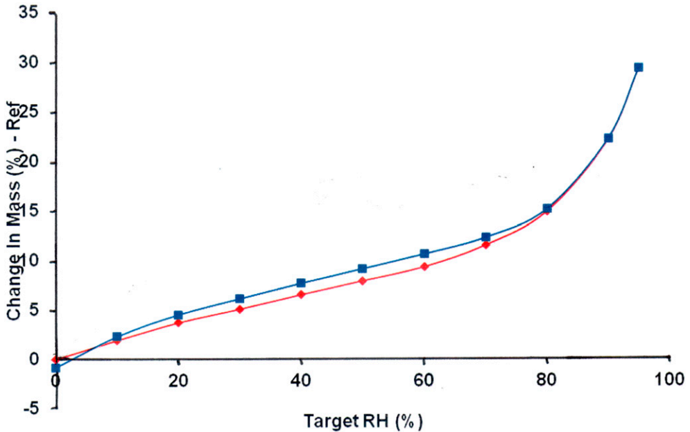
Figure 8. Sorption-desorption isotherms of hair treated with product 2.
