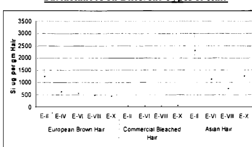
Figure 2: Deposition of Large Silicone Particles from Surfactant A on Different Types of Hair
