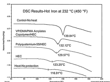
Figure 4-DSC Results
