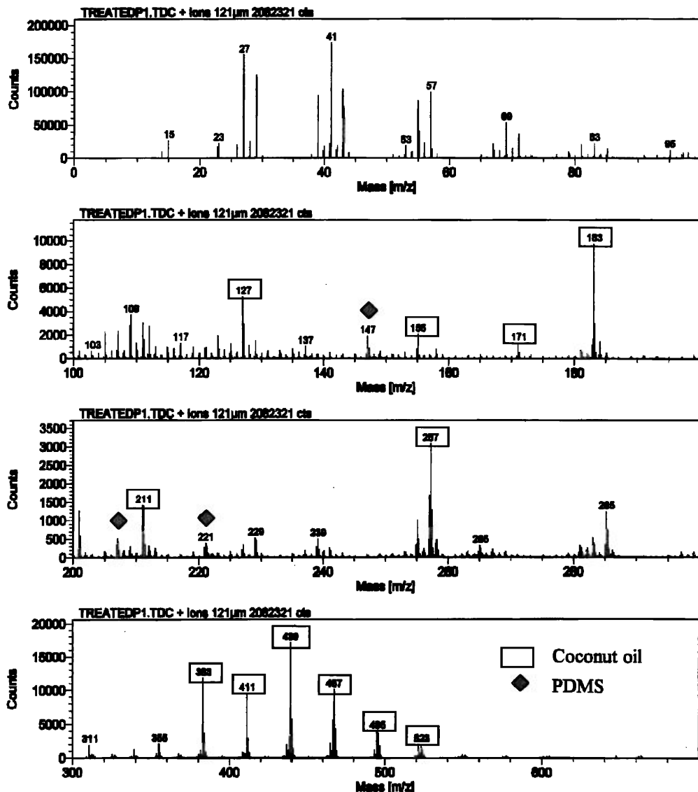
Figure 9. Spectra of positive ions from the surface of a cross section of mineral-oil-treated hair fibers. No characteristic positive ions of mineral oil were detected within mineral-oil-treated hair fibers. However, there is contamination from coconut oil and polydimethylsiloxane surfactants.
